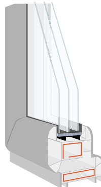
Triple Glazed
